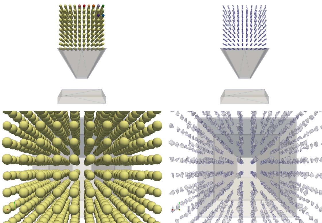
Figure 3.1: Depiction of the two hopper experiments at the starting point. Three types of particles dominate the simulation, a hopper, a floor and the particles. Gravity acceleration is applied to the particles to force them flow through the hopper top and bottom openings. Left: Sphere particles. Right: Triangulated particles (1000 particles made of 5 to 10 triangles).
