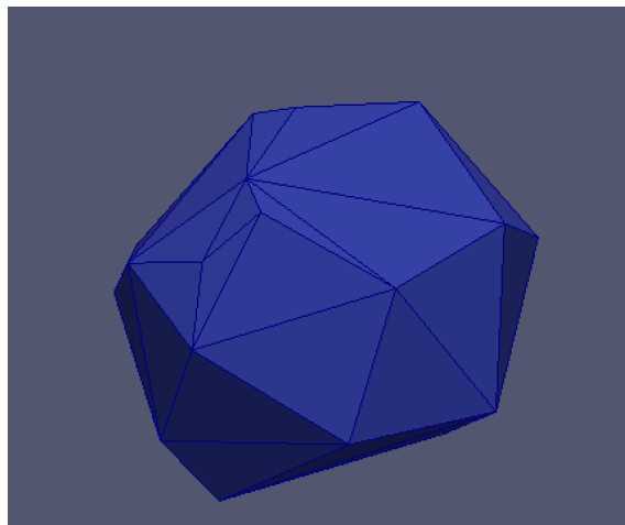
Figure 2.2: A non-spherical triangulated particle approximating a granular material (i.e crushed gravel aggregate).
